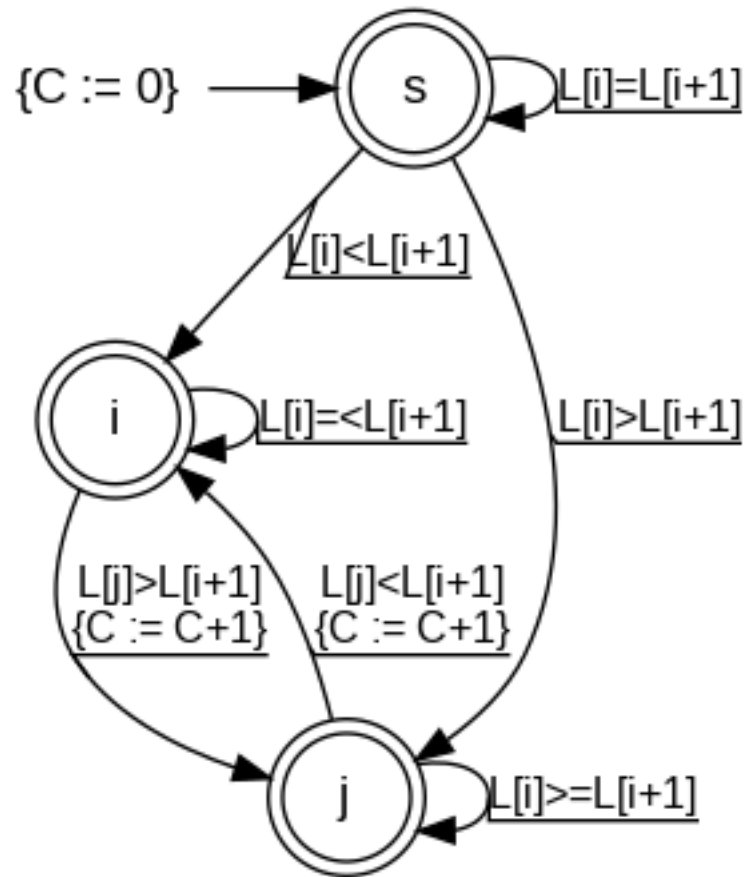
Automaton for inflexion/3 .
