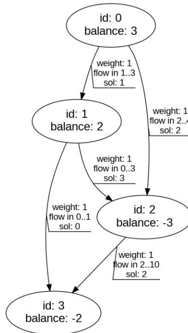
An example of network_flow/3 .
